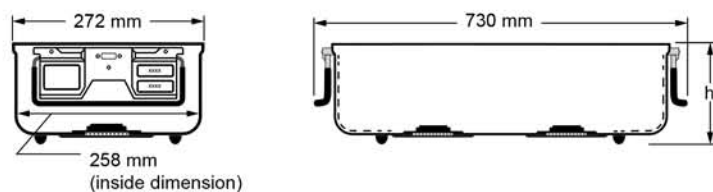
outside dimension
