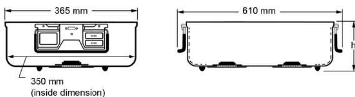
outside dimension
