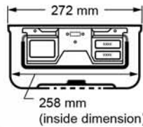
outside dimension
